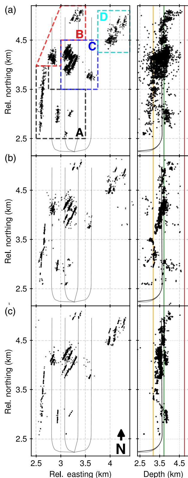
Figure 3. (a) Catalog locations, (b) event-pair relocations, and (c) double-pair relocations for both map view (left) and in-depth (right). Colored lines indicate interfaces for various geologic formations. Injection well outlines (black lines) are also shown. Zones A–D, identified by the dashed polygons, indicate zones of seismicity with similar features. The color version of this figure is available only in the electronic edition.
