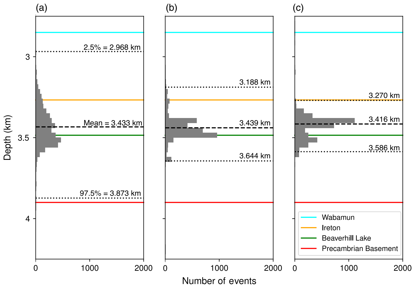
Figure 6. Histograms of hypocenter depths for (a) catalog, (b) event-pair relocations, and (c) double-pair relocations annotated with the 2.5% depth, mean depth, and 97.5% depth intervals for each catalog and notable depth intervals color-coded to match the stratigraphic column (Fig. 2d). The color version of this figure is available only in the electronic edition.
